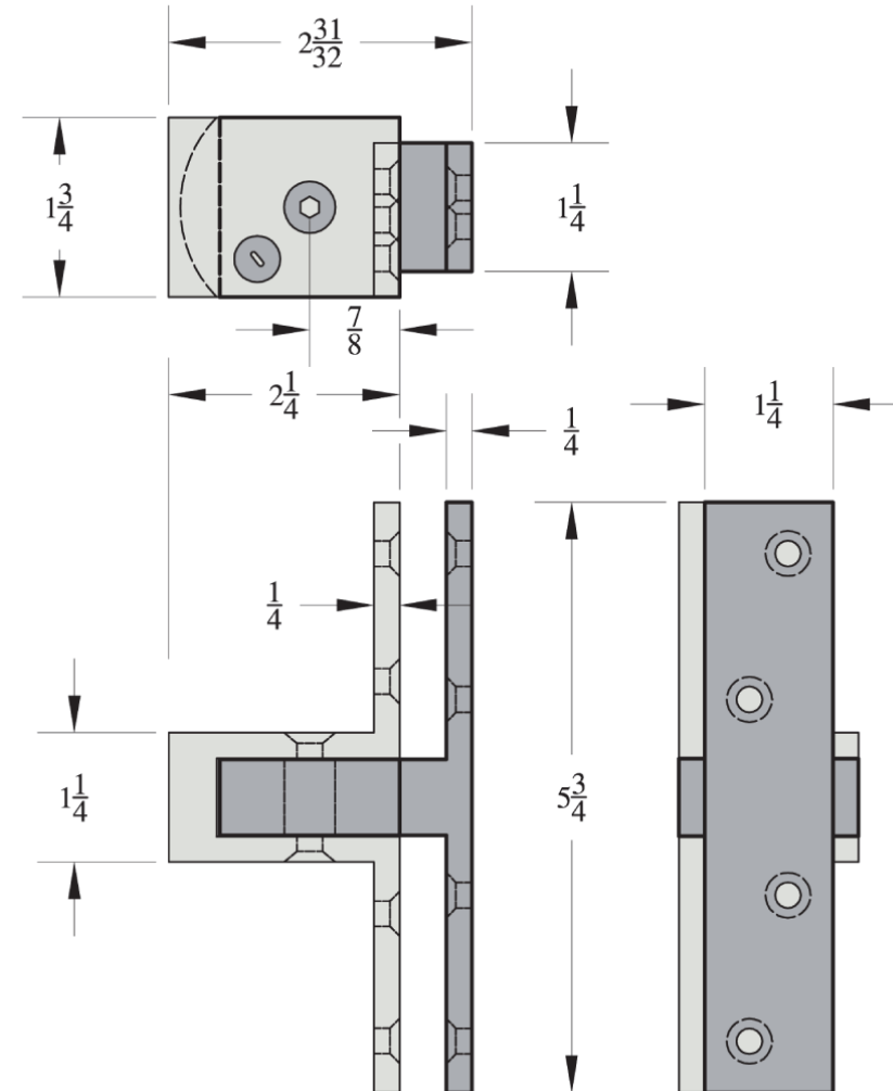
For 1 3/4" Thick Doors
