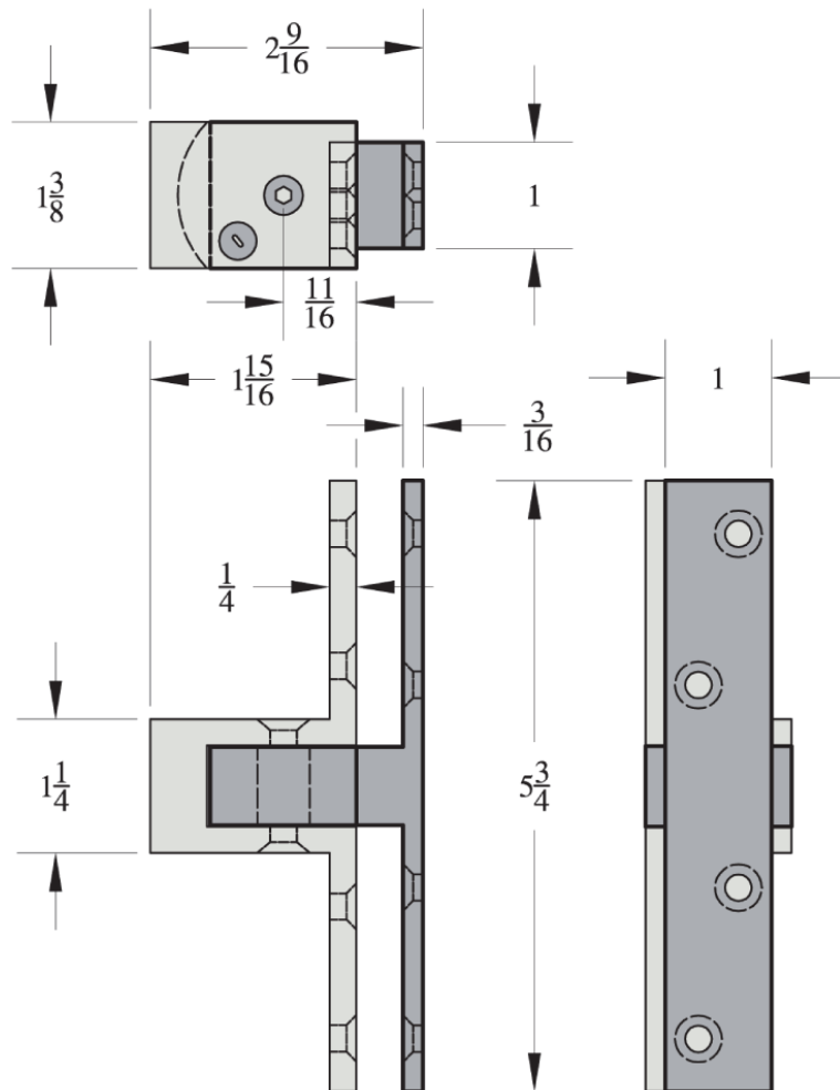
For 1 3/8" Thick Doors
