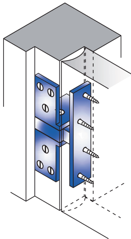
Door in closed position
