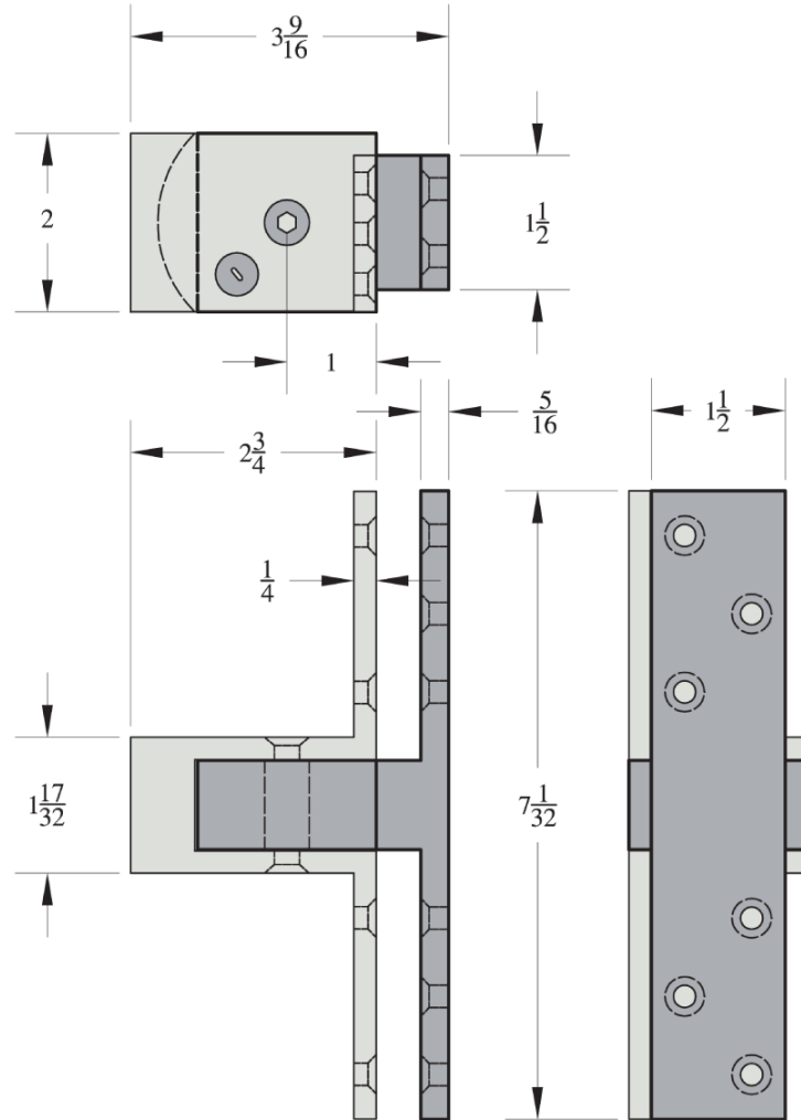
For 2" Thick Doors
