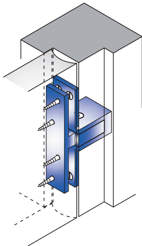
Door in open or "pocket" position
